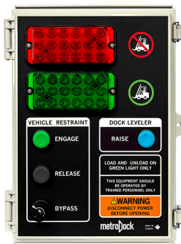
Electric Hook Restraint and Dock Leveler
