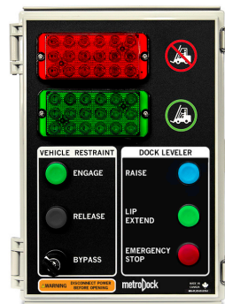
Electric Hook Restraint and Dock Leveler (Raise, Lip Extend, Emergency Stop)
